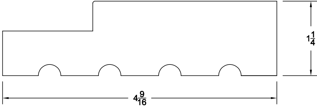
Rabbeted Jamb
