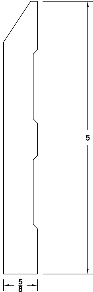
ASM 1201 Baseboard Chamfer
