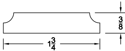
ASM 1611 1 \frac{3}{4} Cove Shoe Mould
